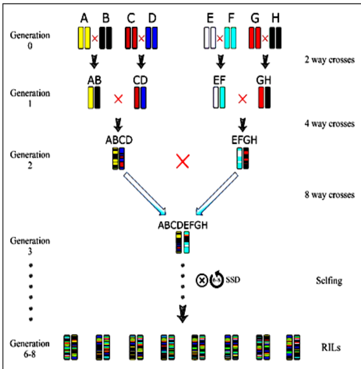
Figure 1: Cross-Designs of a 4-way MAGIC Population.
