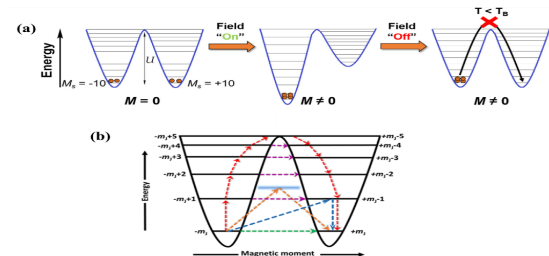
Figure 4: (a) Representation of the spin sublevels for molecules with bistable spin state in absence of an external magnetic field (left); on the application of an external magnetic field, -m_s states are stabilized and all the molecules occupy this spin state (middle); once the field is switched off, the +m_s and -m_s states are degenerate and molecules have to possess U_{\text{eff}} amount of energy to relax their spin state. The figure is obtained from reference [69]. (b) Various possible pathways associated to relaxation of magnetisation for the magnetised molecules. The green arrow represents the ground state quantum tunnelling of magnetisation occurs in the ground state +m_J/-m_J sublevels, while purple arrows represent QTM occurring at higher m_J sublevels known as thermally assisted quantum tunnelling of magnetisation (TA-QTM). The orange arrows represent Raman processes that occur via the formation of a virtual excited m_J state (showing in light blue). Thus, Raman process is a two-phonon phenomenon. The red and blue arrows represent the Orbach process at different energy sublevels. The figure is obtained from reference [70].
