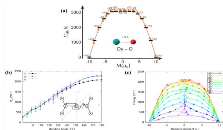
Figure 3: (a) Barrier for spin reversal in one coordinated [\text{DyO}]^+ ion at equilibrium geometry, obtained from reference [39]. (b) The variation of U_{\text{eff}} for a model two coordinated complex, (\text{DyER}_2)_2 as a function of the bending angle ( \angle\text{E-Dy-E} ) \theta and the respective energy levels are shown in figure (c). Obtained from reference [40].
