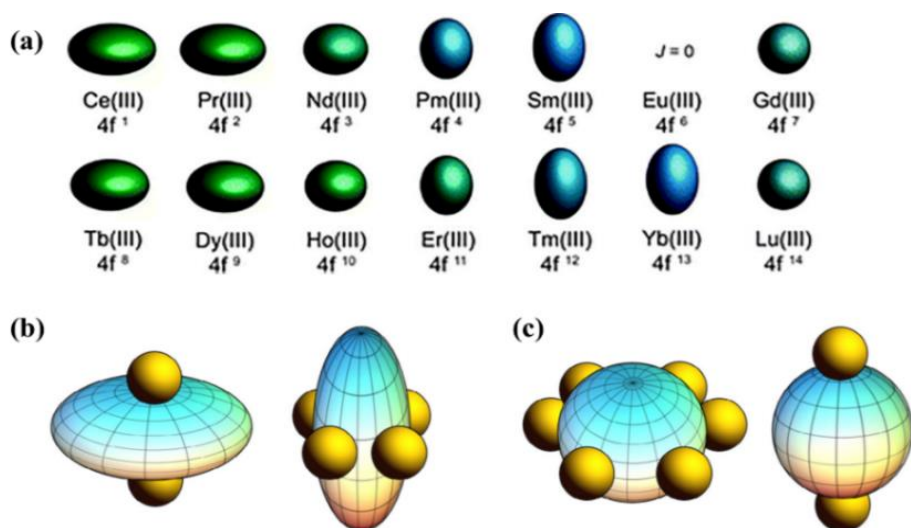
Figure 2: (a) Overall shape of free-ion electron density for Ln(III) ions; oblate, prolate and isotropic shaped ions are shown in different colours. Obtained from reference [37] (b-c) Pictorial representation of ligand field w.r.t. oblate and prolate Ln(III) ions to (b) enhance and (c) quench the magnetic anisotropy.
