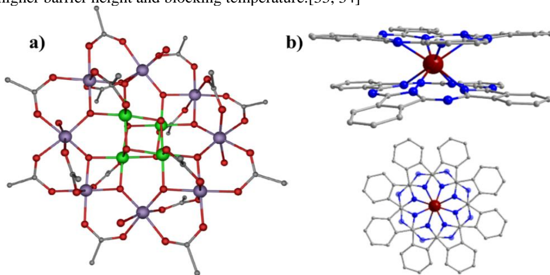
Figure 1: (a) Structure of dodecanuclear mixed valent Mn III /Mn IV cluster, which consists of four Mn IV centres (shown in green) and eight Mn III centres (shown in purple).[1] (b) Structure of [Pc 2 Ln] - ion, Ln: Tb(III) and Dy(III), where two Pc 2- ligands sandwiches the Ln(III) centre.[32]
