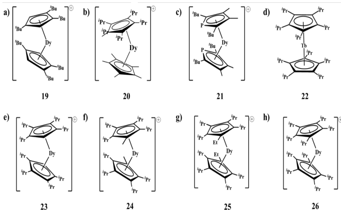
Figure 7: Molecular structures the cationic part of 19-26 (a-h). The counter anions are omitted for clarity. Molecule 20 possesses highest blocking temperature among all the single-molecule magnets.
