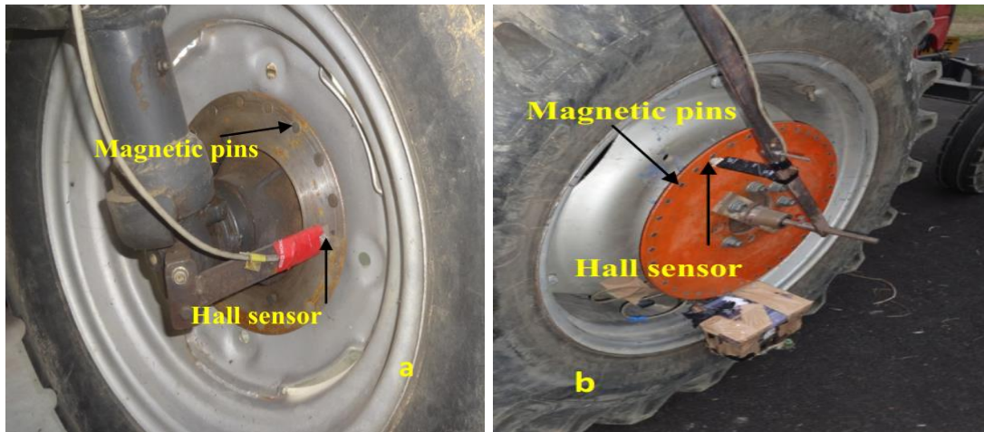
Figure 2: (a) Actual speed measurement (b) Theoretical speed measurement (Source: Kumar et al., 2016)
