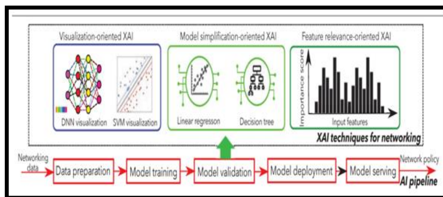
Figure 5: AI Pipeline for XAI Techniques for Networking
