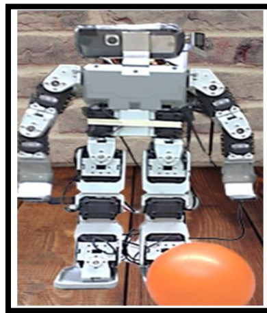
Figure 9: Modified Robotis Bioloid Robot
