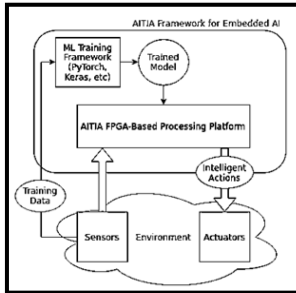
Figure 7: The Working of AITIA
