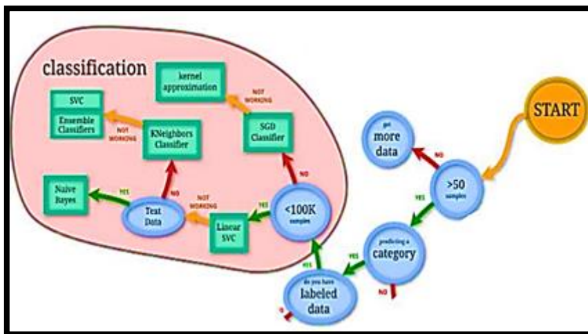
Fig 3: Classifier Model Flowchart
