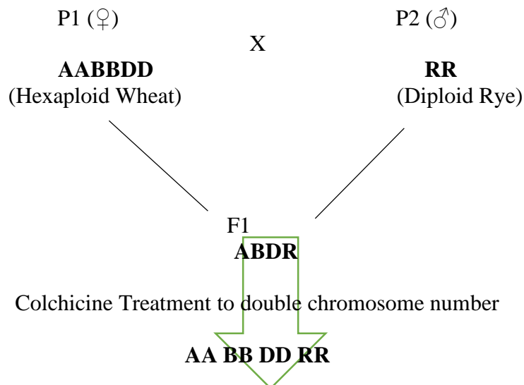
Figure 2: Primary Octoploid Triticale
