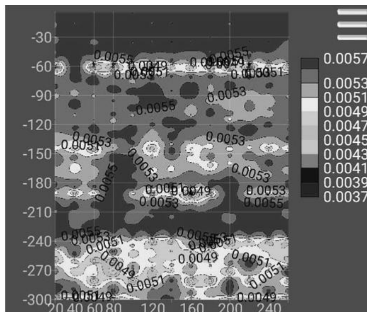
Figure 2.2: MT Profile 2
