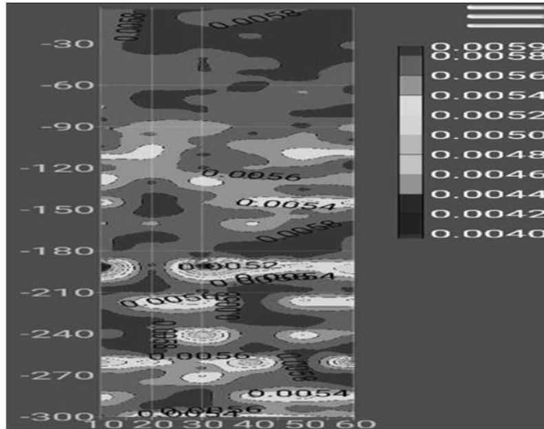
Figure 2.3: MT profile 3
