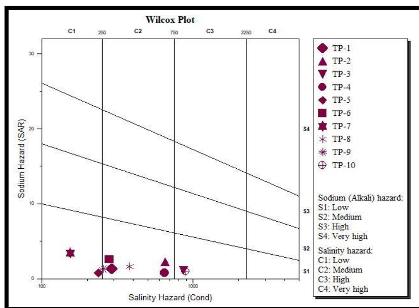
Figure 5: Wilcox Plot.
