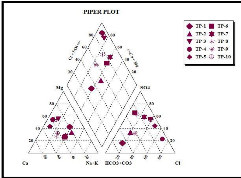
Figure 4: Piper Plot
