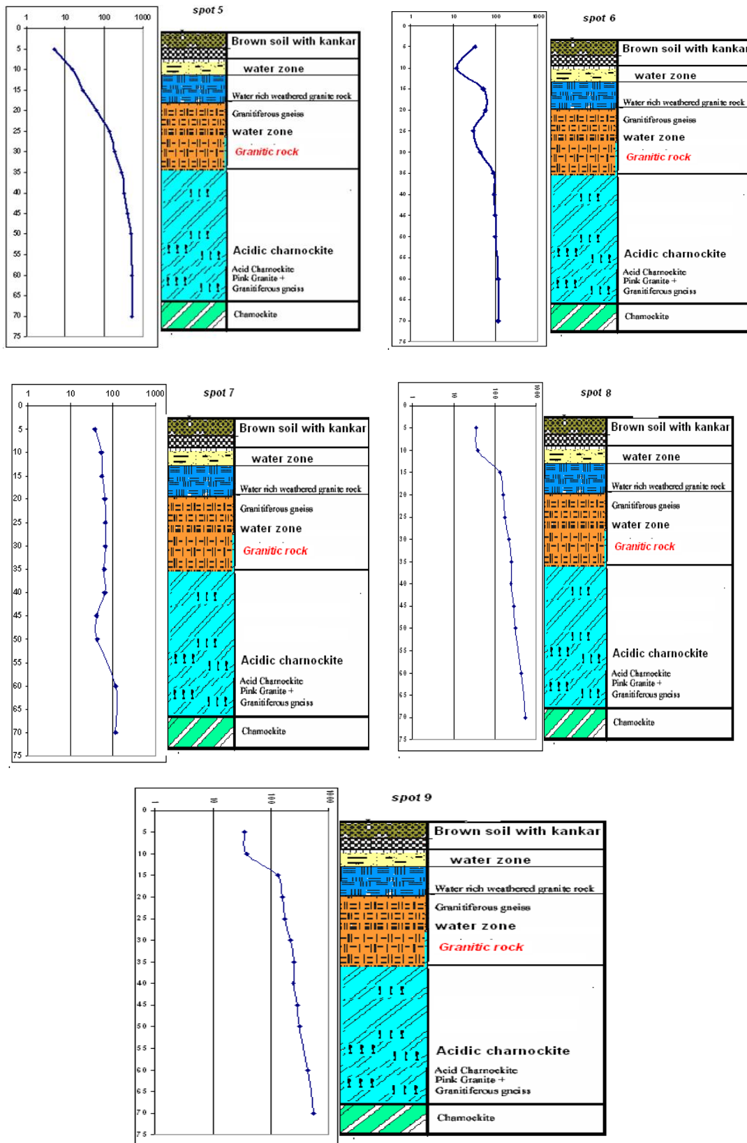
Figure 3: Apparent Resistivity VS Depth plot and Lithology.
