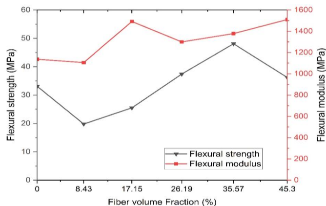
Figure 2: Variation of flexural properties based on the fiber loading in FSP fiber/vinyl ester composites
