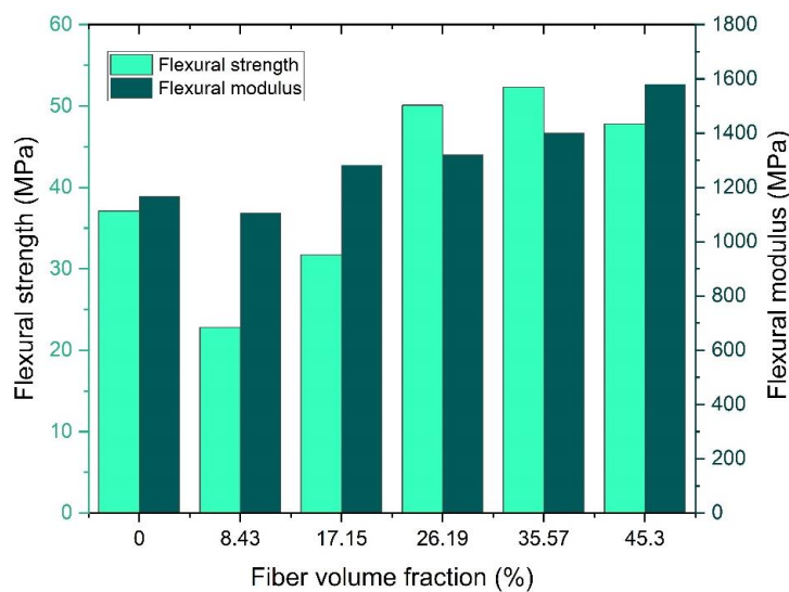
Figure 5: Variation of flexural properties based on the fiber loading in FSP fiber/vinyl ester composites
